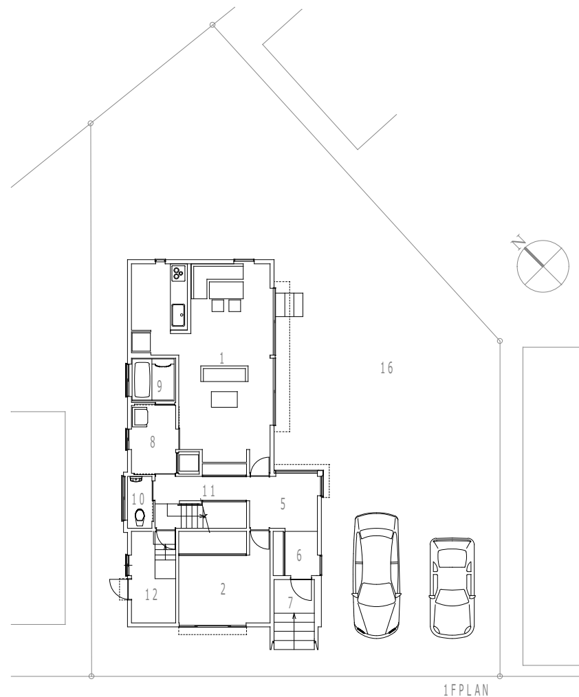
1FPLAN
